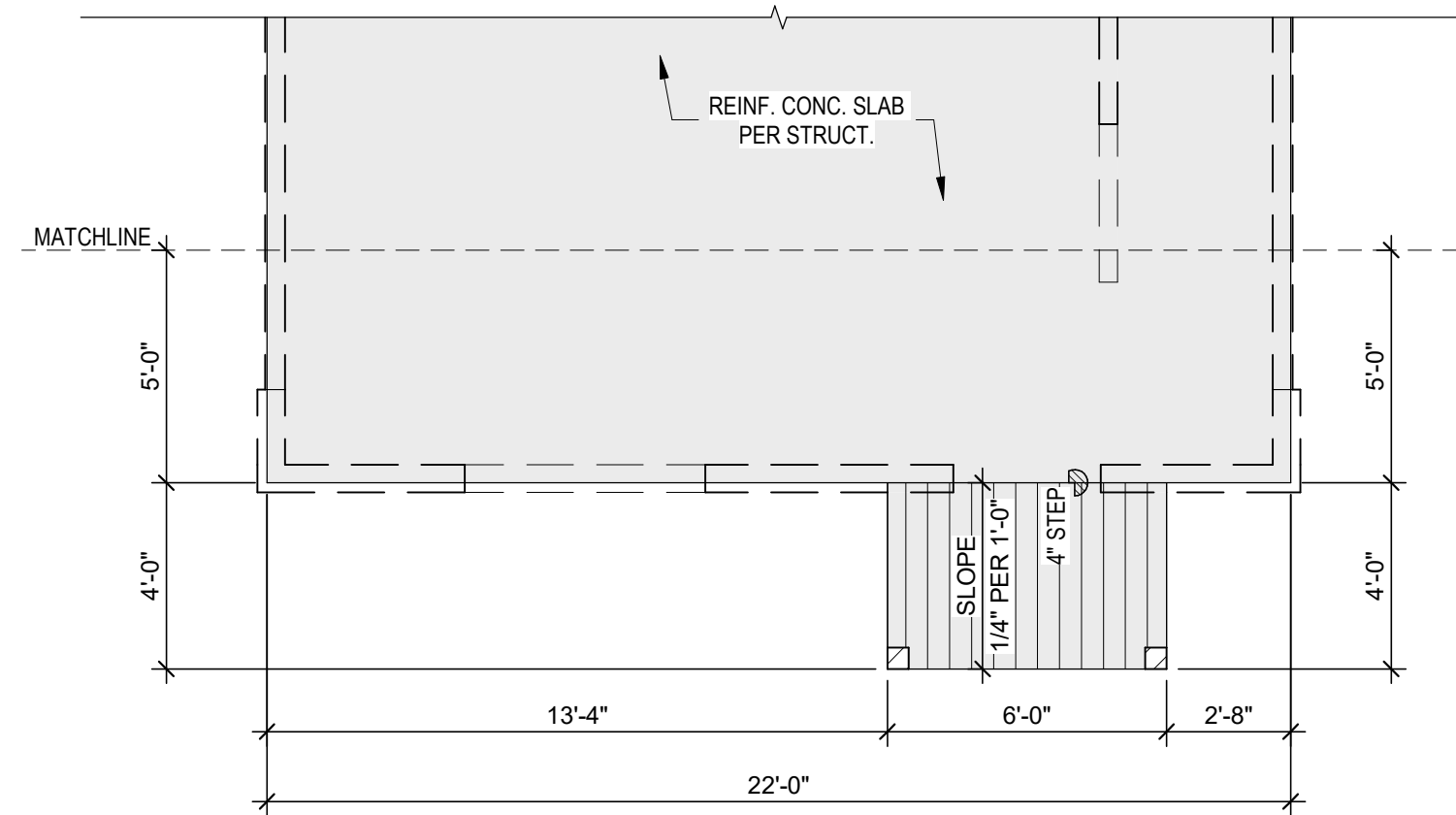
2 SINGLE UNIT - OPTION 2 1/4" = 1'-0"
