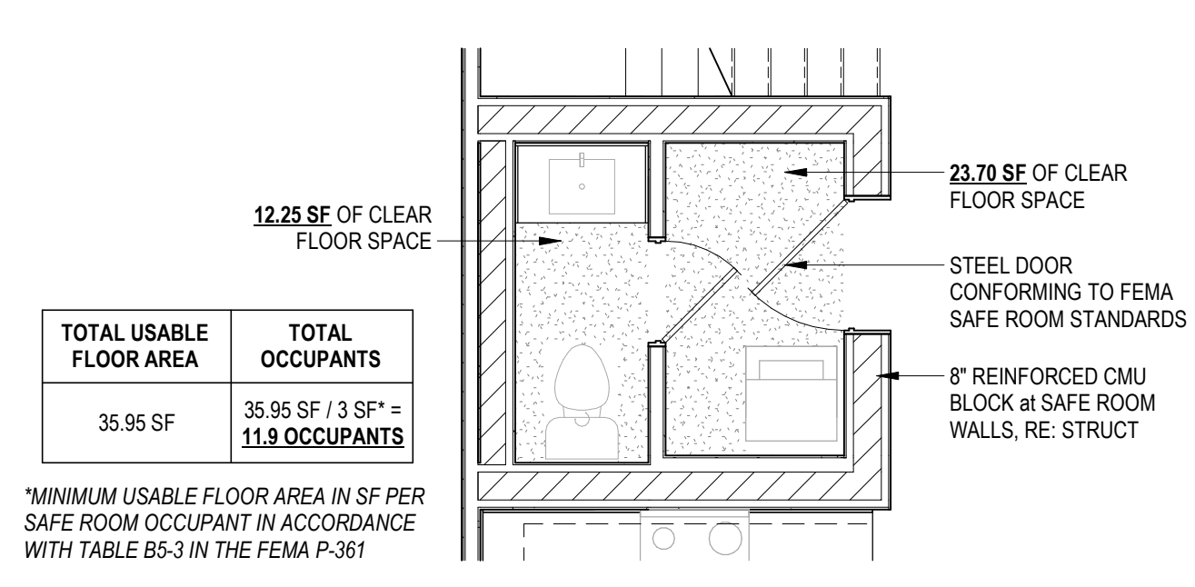
6 FEMA SAFE ROOM PLAN 1/4" = 1'-0"
